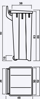
MISURE D'INGOMBRO - OVERALL DIMENSIONS
